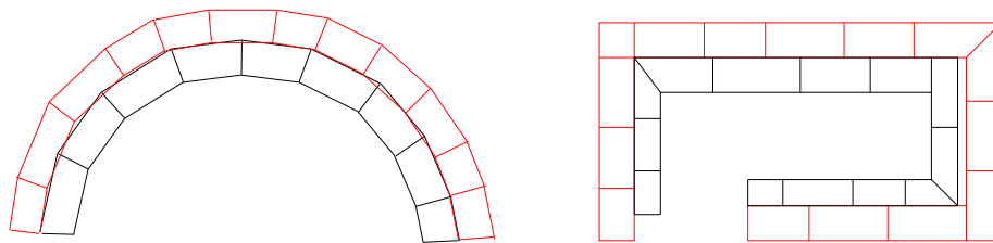
Figure VII.B.7: Initial surfaces
