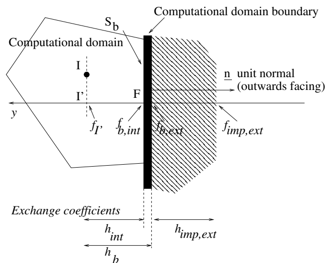
Figure IV.C.1: Boundary cell.
