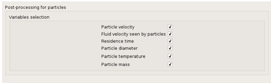
Figure II.30: Solution controls.
