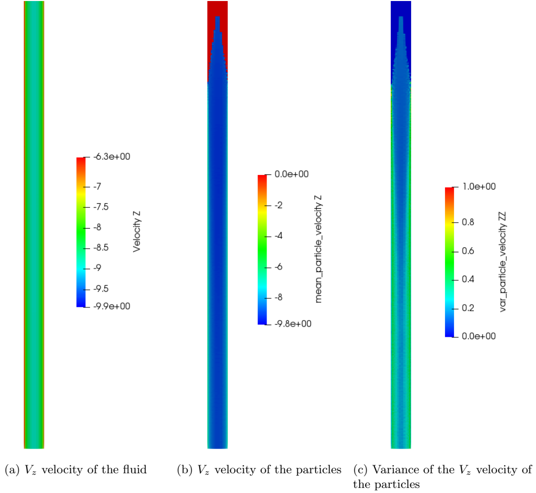
Figure II.39: Visualization in the yz plane along the pipe axis
