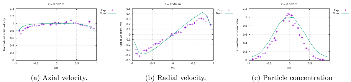
Figure II.41: Numerical (line) and experimental[4] (symbols) results at z = 0.502m .
