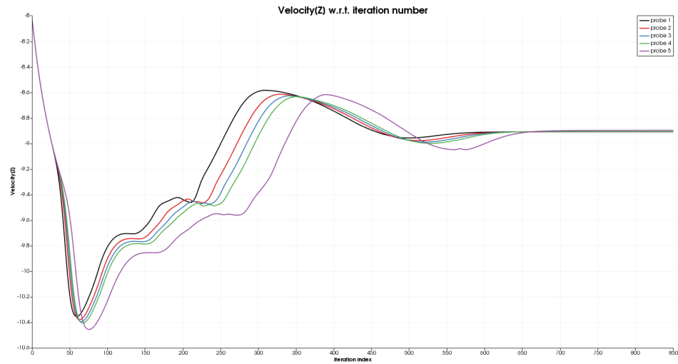
Figure II.23: Evolution of axial velocity during the calculation
