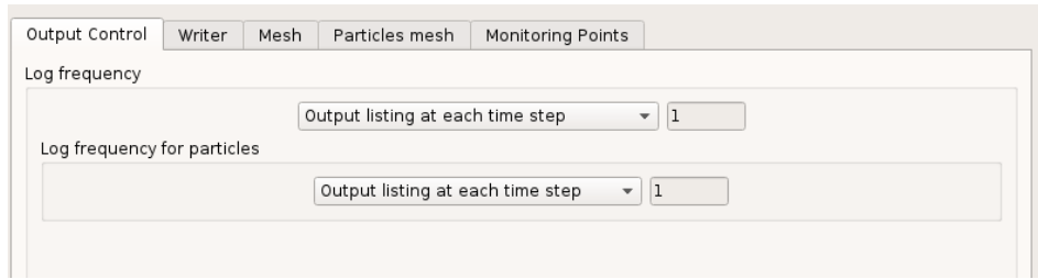
Figure II.29: Output menu.
