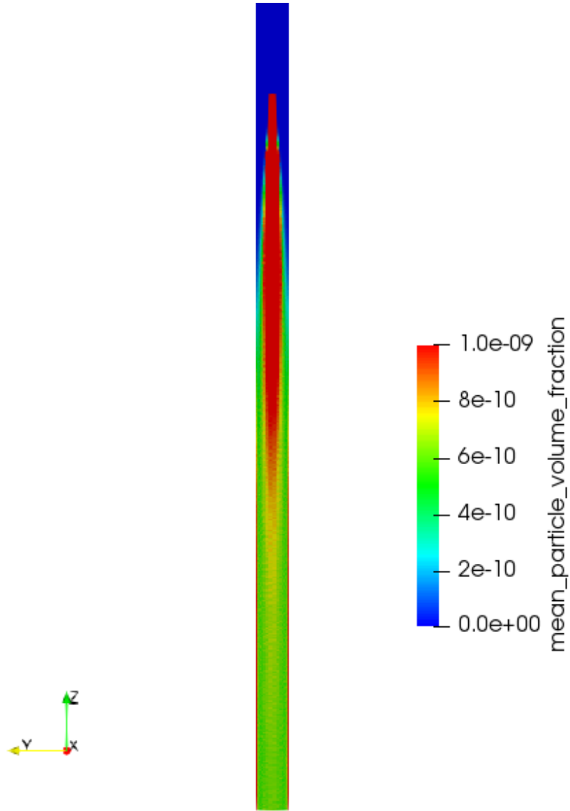
Figure II.38: Volume fraction of the particles in the pipe.
