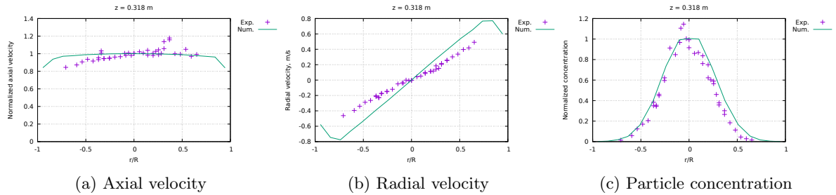
Figure II.40: Numerical (line) and experimental[4] (symbols) results at z = 0.318m .
