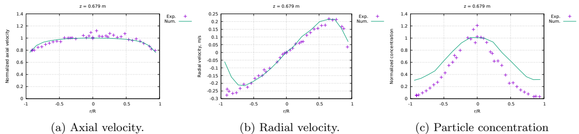
Figure II.42: Numerical (line) and experimental[4] (symbols) results at z = 0.679m .
