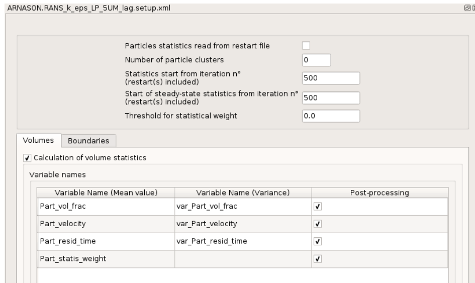
Figure II.28: Statistics menu.
